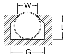
dovetail groove
