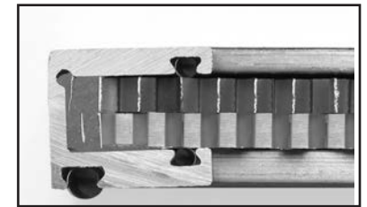
"C" Frame Spiral Bonding (2 panel configuration shown)
