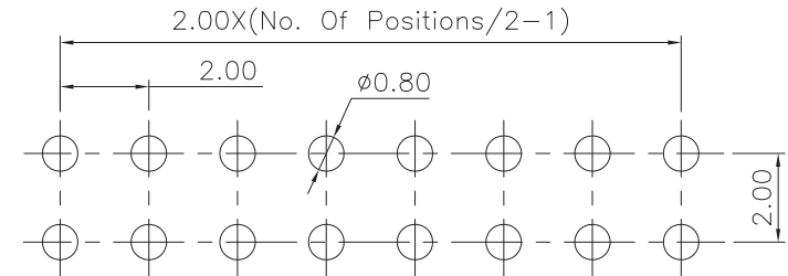
PCB Layout
