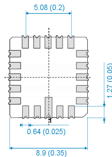
MS9000 bottom view
