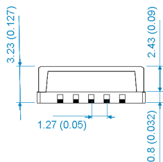
MS9000 side view
