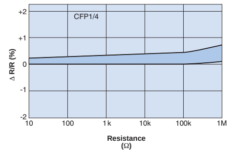
Load Life @ 70°C, 1000 Hr
