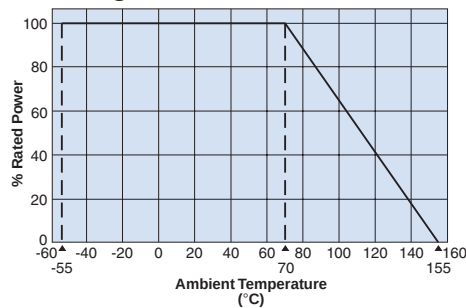
Derating Curve
