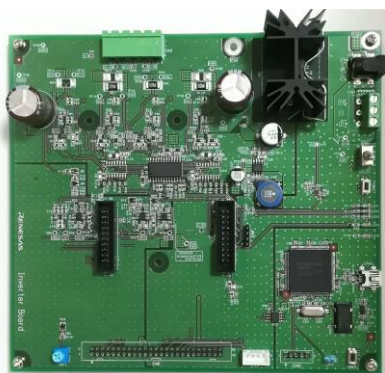
(1) Inverter board
