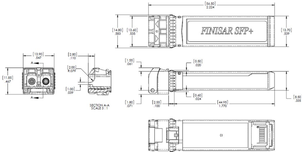
Figure 2. FTLX8574D3BCL Mechanical Dimensions.
