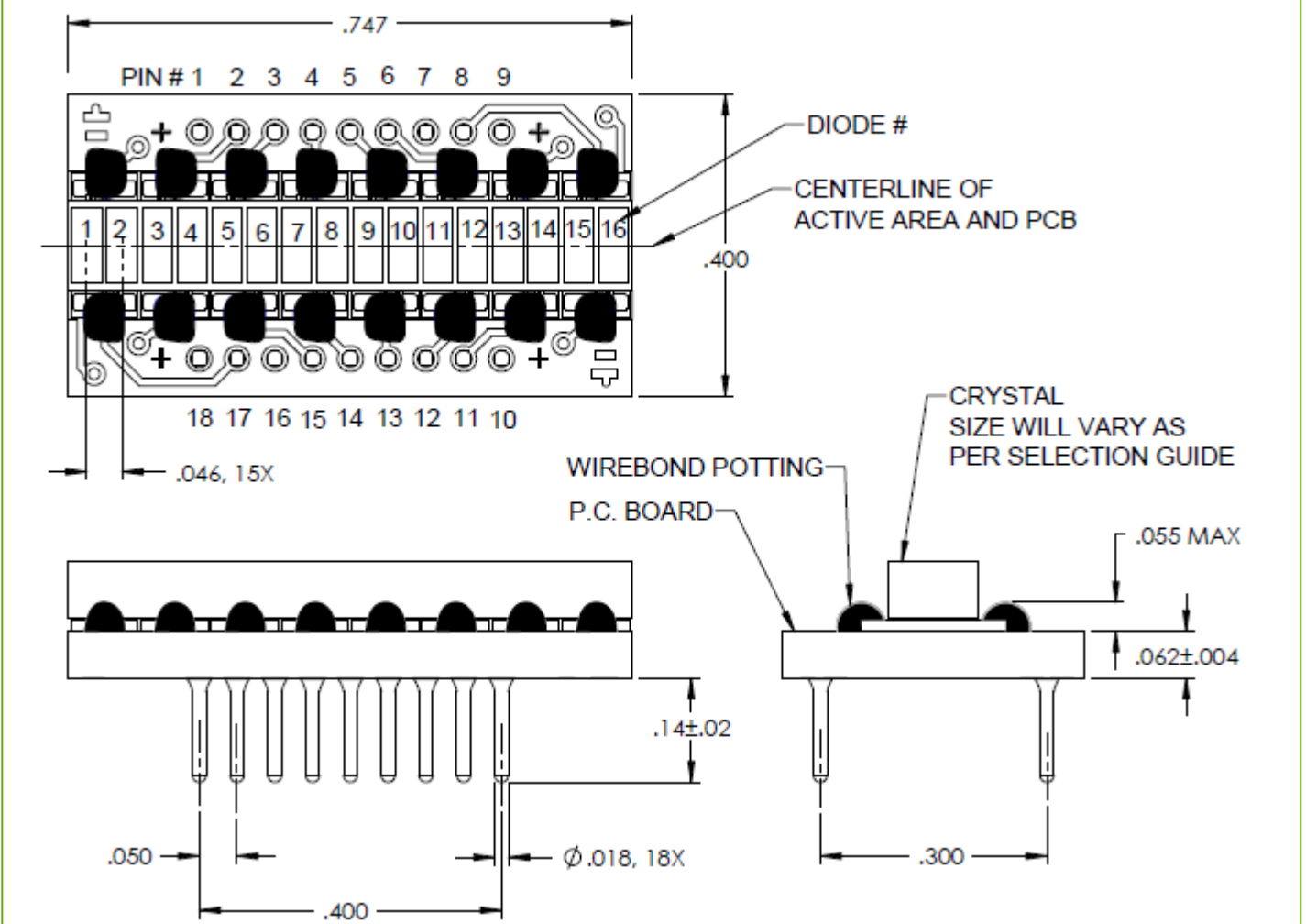
VTA1216H-H (Dimensions are in inches)
