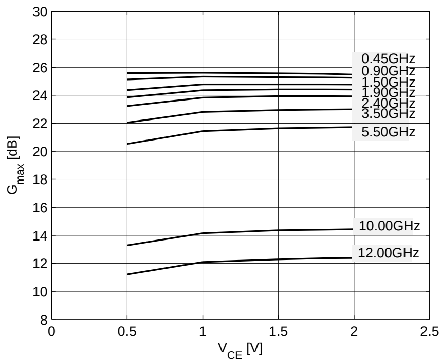
Figure 7-6 Maximum Power Gain G_{\max} = f(V_{CE}) , I_C = 15\text{ mA} , f = \text{Parameter in GHz}
