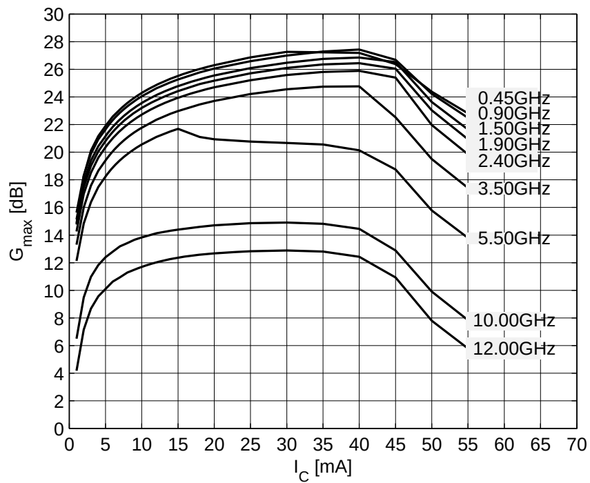
Figure 7-5 Maximum Power Gain G_{\max} = f(I_C) , V_{CE} = 1.8\text{ V} , f = \text{Parameter in GHz}
