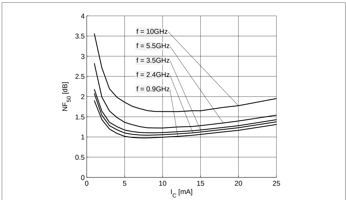
Figure 7-12 Noise Figure NF_{50} = f(I_C) , V_{CE} = 1.8 V, Z_S = 50 \Omega , f = Parameter in GHz
