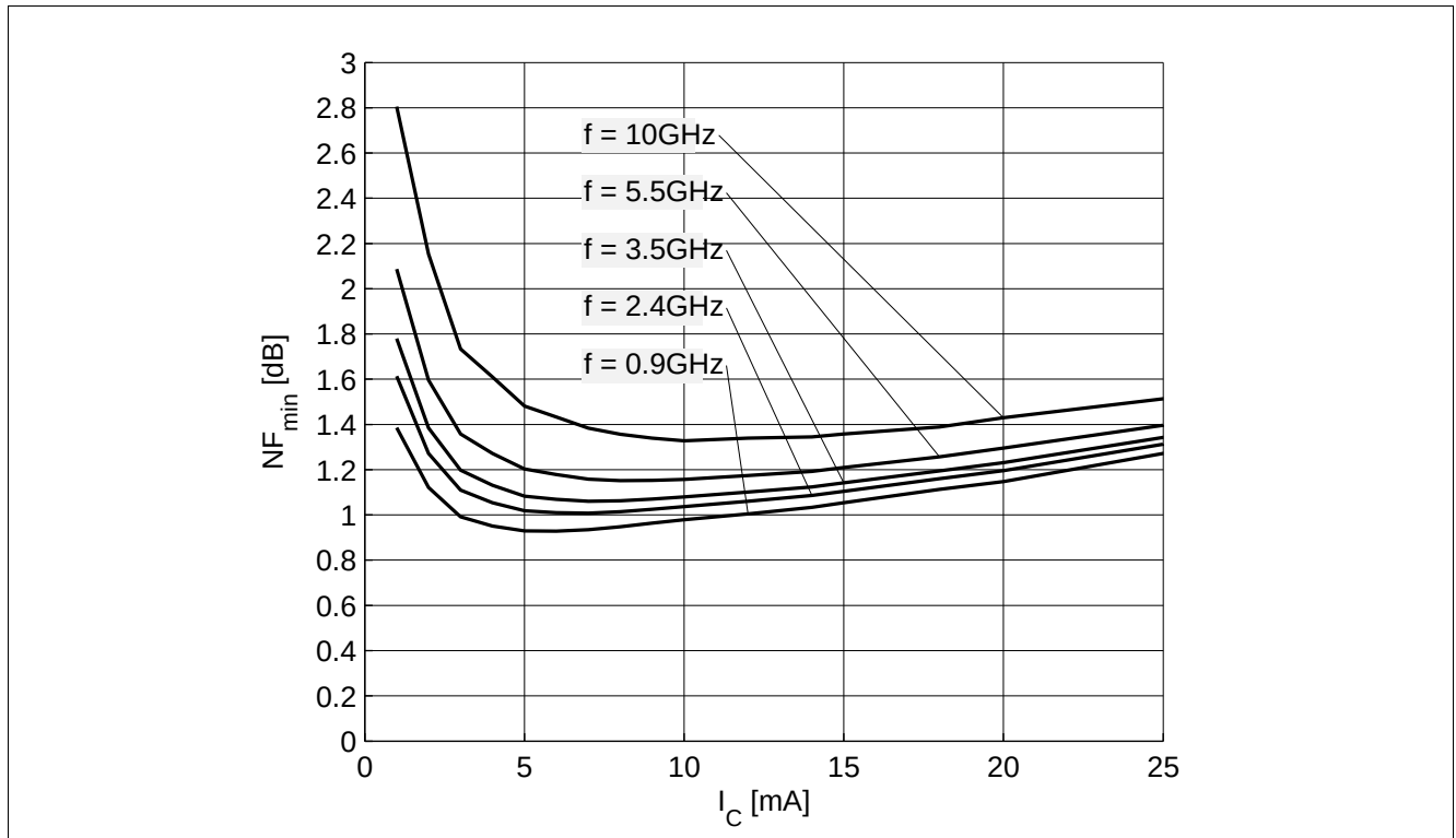
Figure 7-11 Noise Figure NF_{min} = f(I_C) , V_{CE} = 1.8 V, Z_S = Z_{opt} , f = Parameter in GHz
