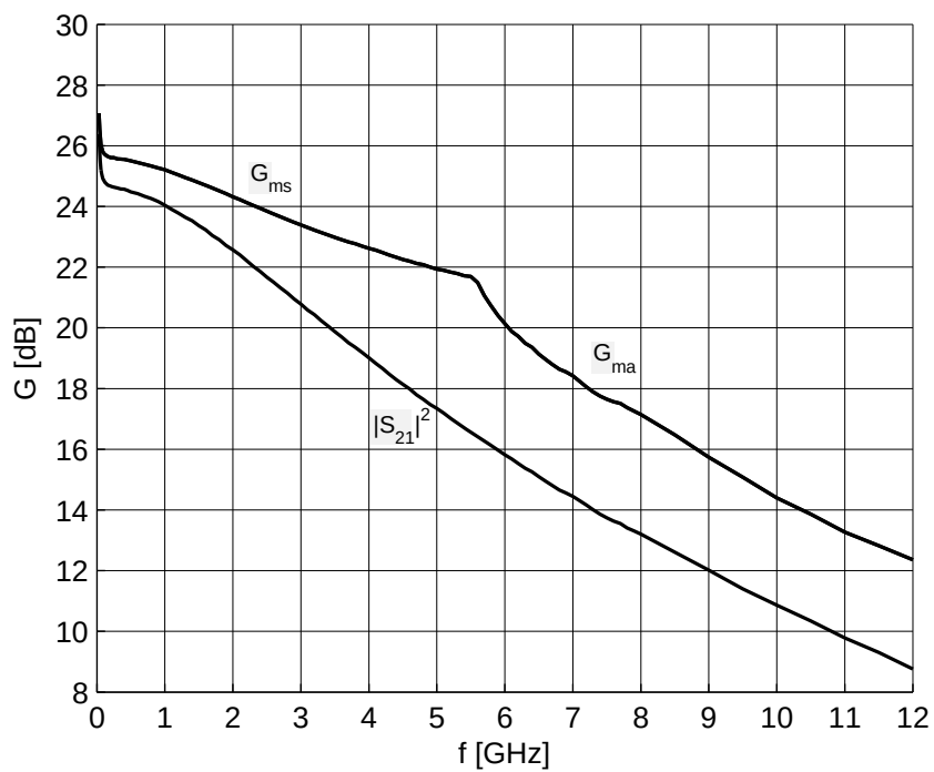
Figure 7-4 Gain G_{ma} , G_{ms} , |S_{21}|^2 = f(f) , V_{CE} = 1.8 \text{ V} , I_C = 15 \text{ mA}
