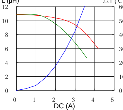
11. RCR875DNP-120L
