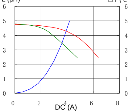
9. RCR875DNP-8R2L
