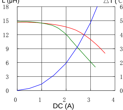
12. RCR875DNP-150L
