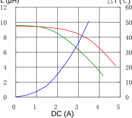
10. RCR875DNP-100L
