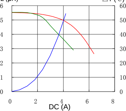
10. RCR875DNP-100L
