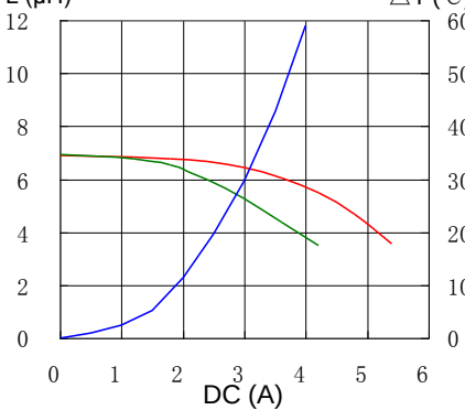
11. RCR875DNP-120L
