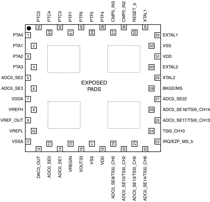
Figure 20. 44-pin Laminite QFN
