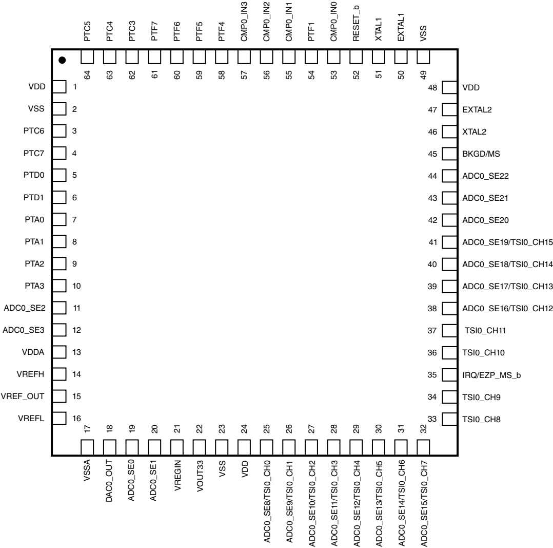
Figure 18. 64-pin LQFP
