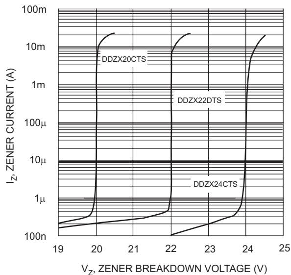
Fig. 7 Typical Reverse Characteristics, DDZX20CTS - DDZX24CTS
