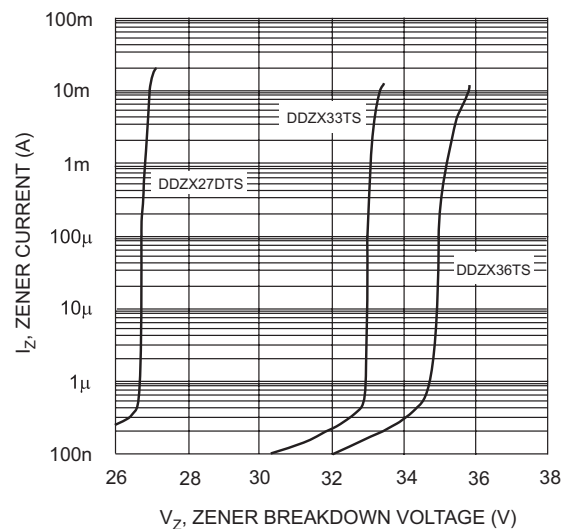
Fig. 8 Typical Reverse Characteristics, DDZX27DTS - DDZX36TS
