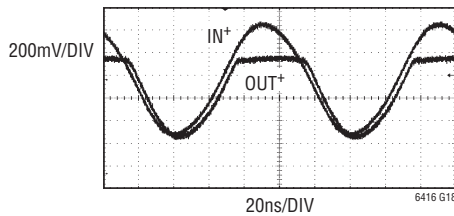
Positive Overdrive Recovery ( V_{CLHI} Pin)
