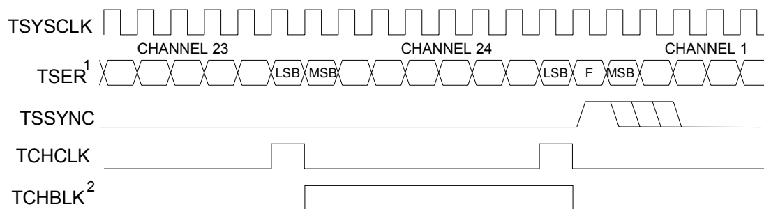
Figure 35-20. Transmit-Side Boundary Timing, TSYSCLK = 1.544MHz (Elastic Store Enabled)
