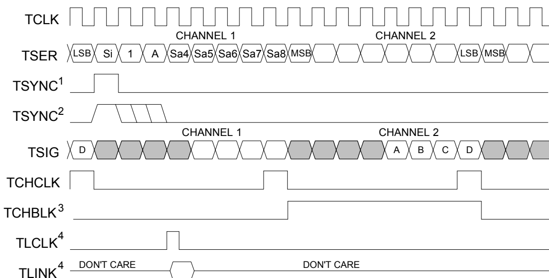
Figure 35-19. Transmit-Side Boundary Timing (Elastic Store Disabled)
