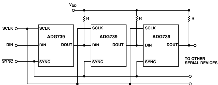
Figure 20. Multiple ADG739 Devices in a Daisy-Chained Configuration
