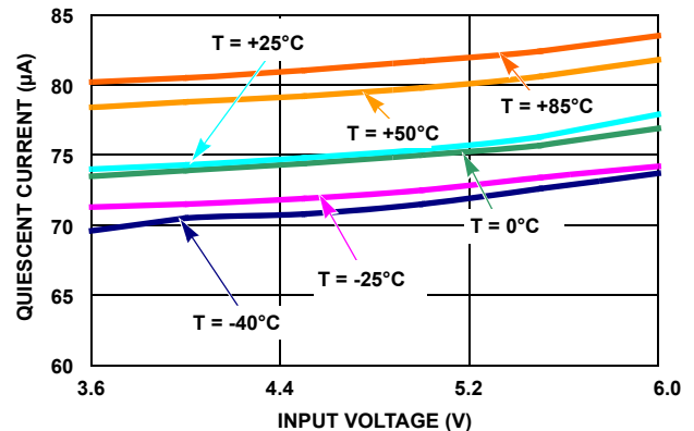
FIGURE 7. QUIESCENT CURRENT vs INPUT VOLTAGE ( V_{OUT1} = V_{OUT2} = 3.3V , LD01 AND LD02 ENABLED)
