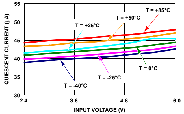
FIGURE 3. QUIESCENT CURRENT vs INPUT VOLTAGE ( V_{OUT2} = 2.1V , ONLY LD02 ENABLED)
