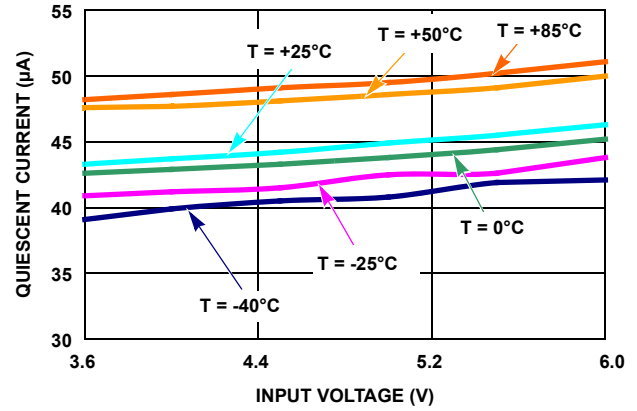
FIGURE 5. QUIESCENT CURRENT vs INPUT VOLTAGE ( V_{OUT1} = 3.3V , ONLY LD01 ENABLED)
