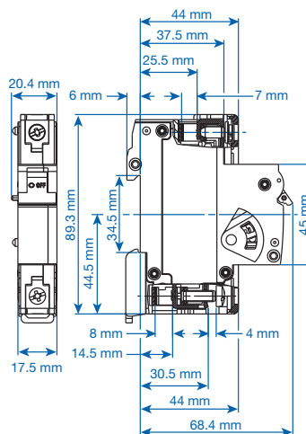
Dimensions FAxxUM, UA120UM, N63UM.
