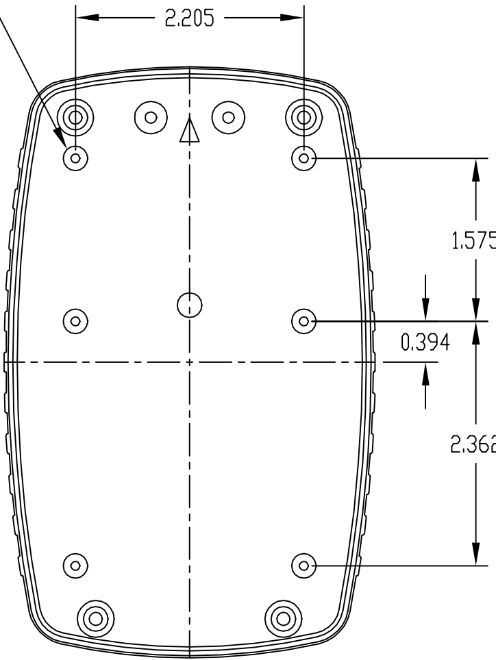
INSIDE VIEW OF BOTTOM
