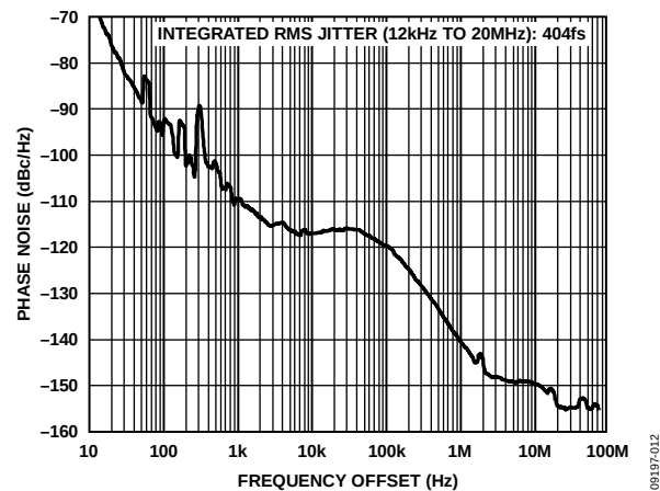
Figure 12. Absolute Phase Noise (Output Driver = HSTL), f_R = 19.44 MHz, f_O = 312.5 MHz, DPLL Loop BW = 0.1 Hz, f_{SYS} = 19.2 MHz TCXO
