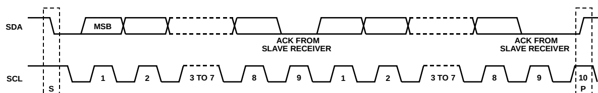
Figure 51. Acknowledge Bit
