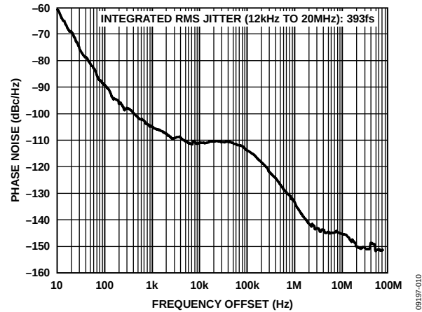
Figure 10. Absolute Phase Noise (Output Driver = HSTL), f_R = 19.44 MHz, f_O = 644.53 MHz, DPLL Loop BW = 0.1 Hz, f_{SYS} = 19.2 MHz TCXO
