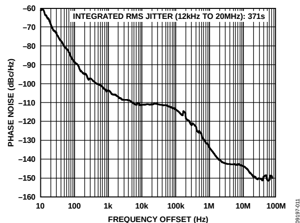
Figure 11. Absolute Phase Noise (Output Driver = HSTL), f_R = 19.44 MHz, f_O = 693.482991 MHz, DPLL Loop BW = 0.1 Hz, f_{SYS} = 19.2 MHz TCXO
