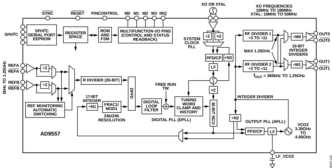
Figure 35. Detailed Block Diagram
