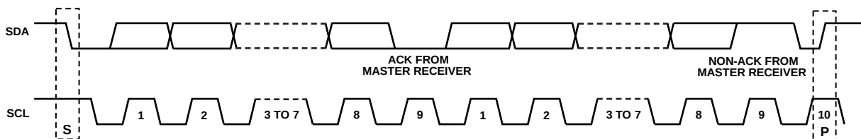
Figure 53. Data Transfer Process (Master Read Mode, 2-Byte Transfer)
