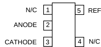
LM4041_ADJH5 (SC70-5)
