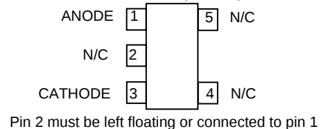
LM4041_H5 (SC70-5)
