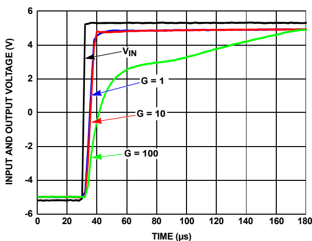
FIGURE 52. NEGATIVE OVERLOAD RECOVERY TIME, ISL2863x
