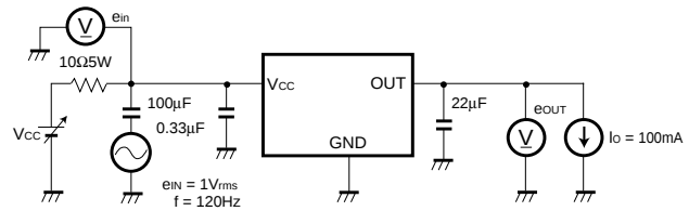
Fig. 2 Measurement circuit for ripple rejection ratio
