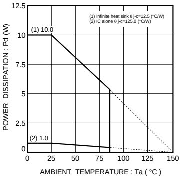
Fig. 7 Ta - power dissipation characteristics (TO 252-3)
