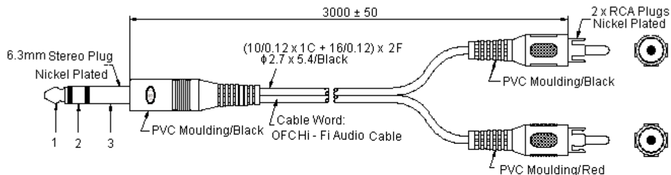
Soldering Drawing:
