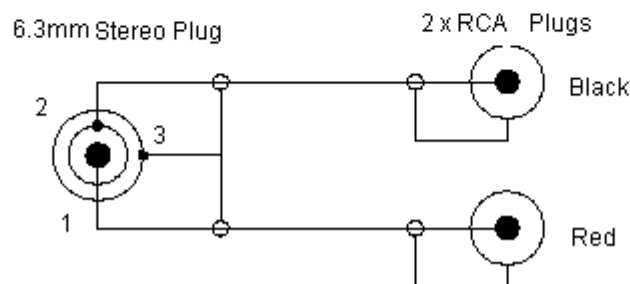
Soldering Drawing:
