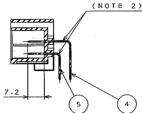
SECT. B-B
