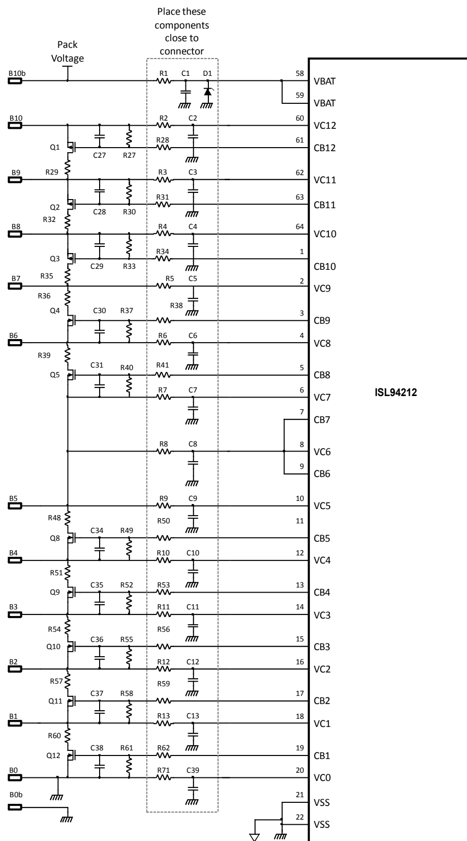
FIGURE 41. BATTERY CONNECTION CIRCUITS, SYSTEM WITH 10 CELLS
