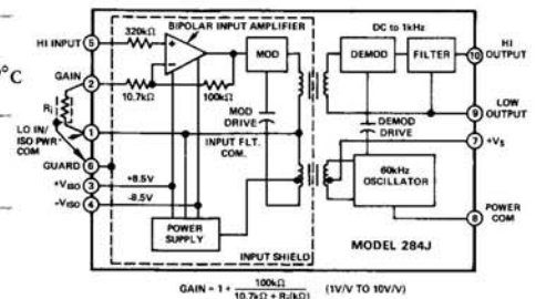
Figure 1. Block Diagram — Model 284J
