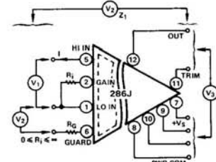
Figure 9. Model 286J Terminal Ratings
