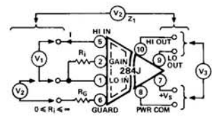
Figure 7. Model 284J Terminal Ratings
