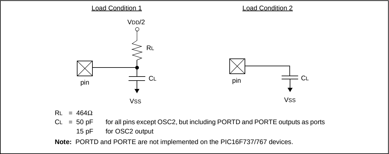
FIGURE 18-4: LOAD CONDITIONS
