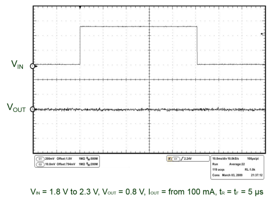
Figure 27. Line transient
