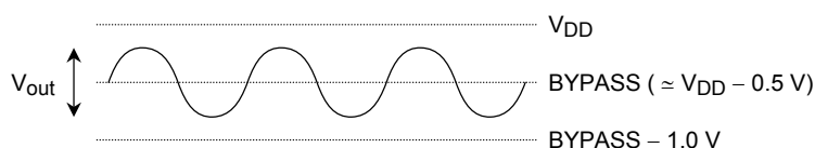
Amp output waveform (AMP0): AMP0_OUT pin
