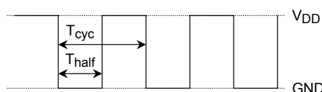
Amp output waveform (AMP1): PSK_RXD pin
