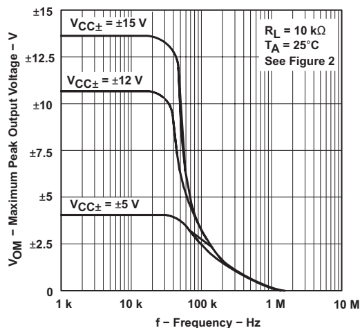
Figure 7. Maximum Peak Output Voltage vs Frequency
