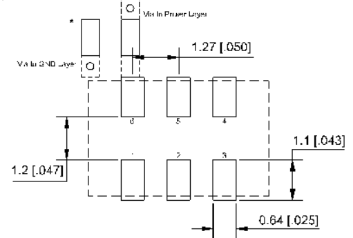
Recommended Solder Pad Layout units: mm[inch]
