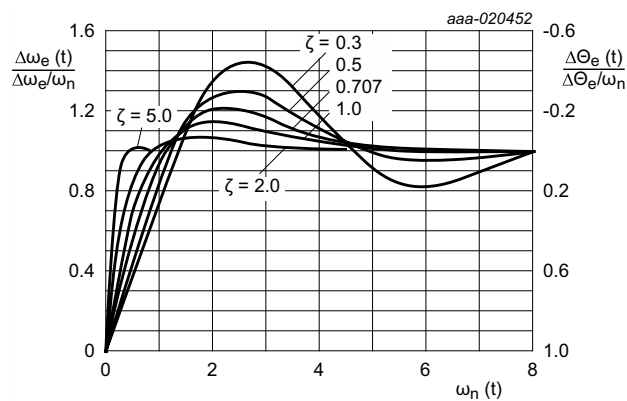
Fig 34. Type 2, second order frequency step response
