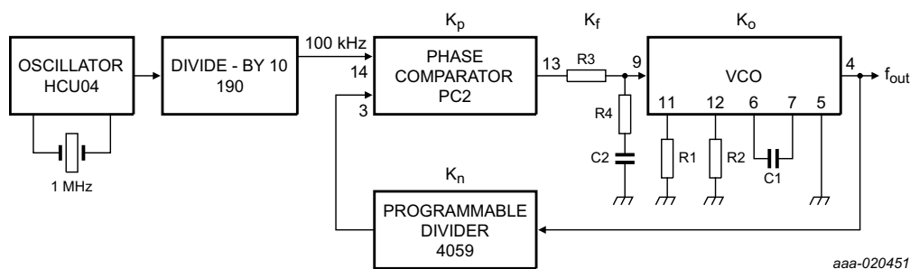
Fig 33. Frequency synthesizer
