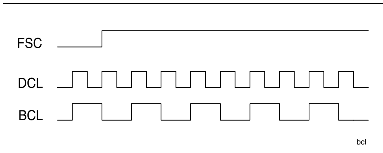
Figure 10 Clock waveforms
