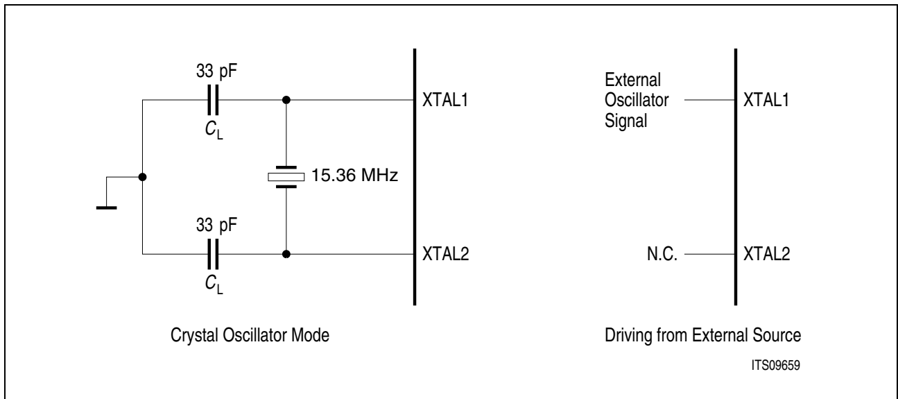
Figure 77 Oscillator Circuit
