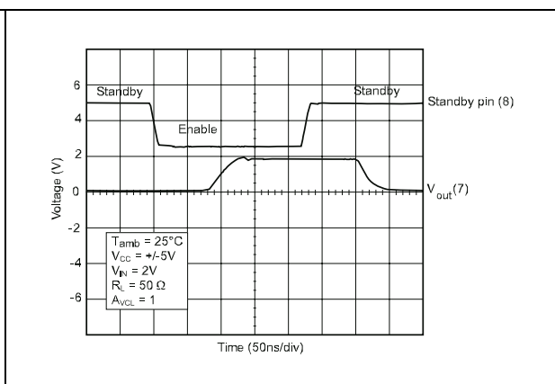
Figure 16. Standby switching
