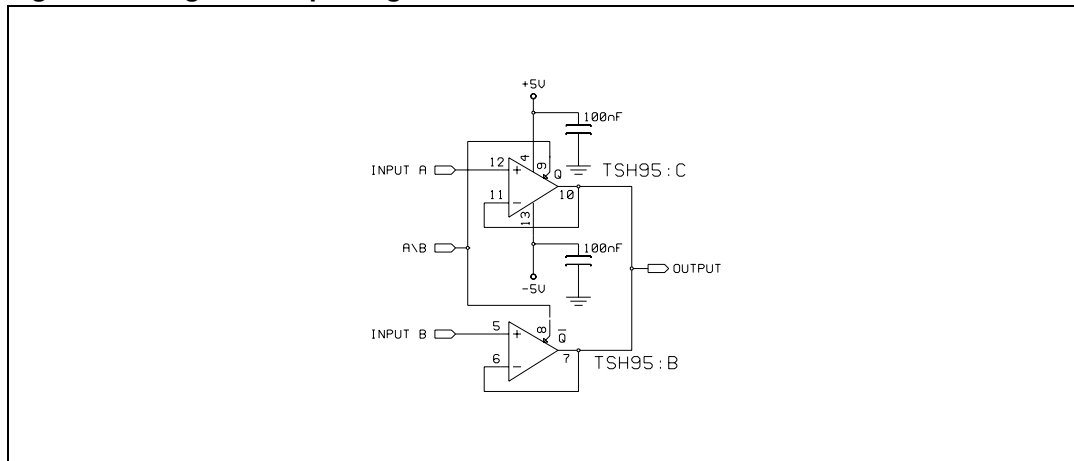
Figure 3. Signal multiplexing
