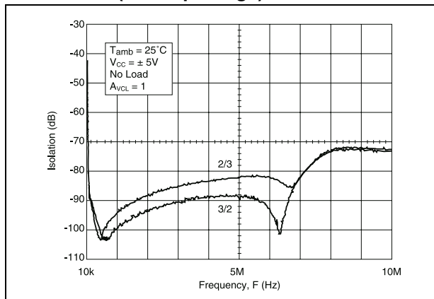
Figure 13. Crosstalk isolation vs. frequency (SO-16 package)
