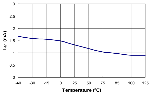
Figure 14. Supply Current Drawn from Pin HV (I HV ) vs. Temperature
