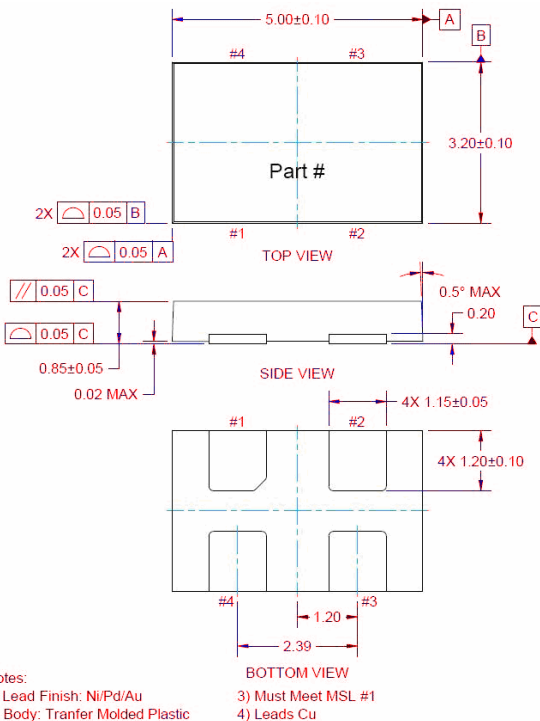
3.2 mm x 5.0 mm x 0.85 mm QFN type package
