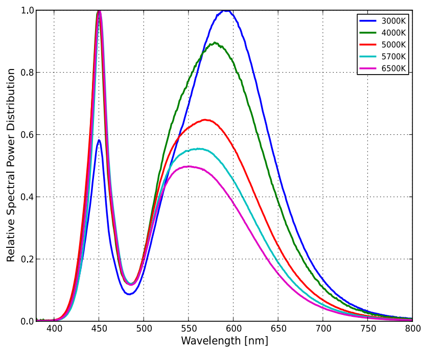
Figure 1a. Typical normalized power vs. wavelength for L130-xx70003000x21 at 120mA, T j =25°C.
