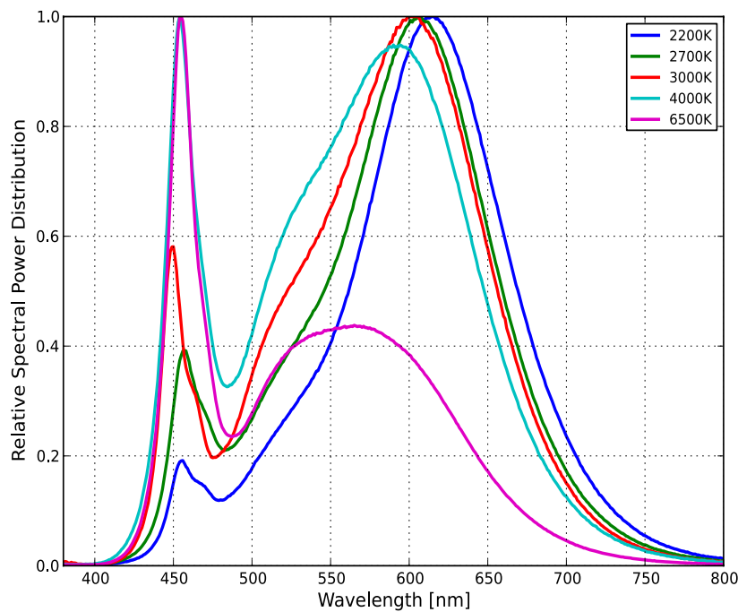
Figure 1b. Typical normalized power vs. wavelength for L130-xx80003000x21 at 120mA, T j =25°C.
