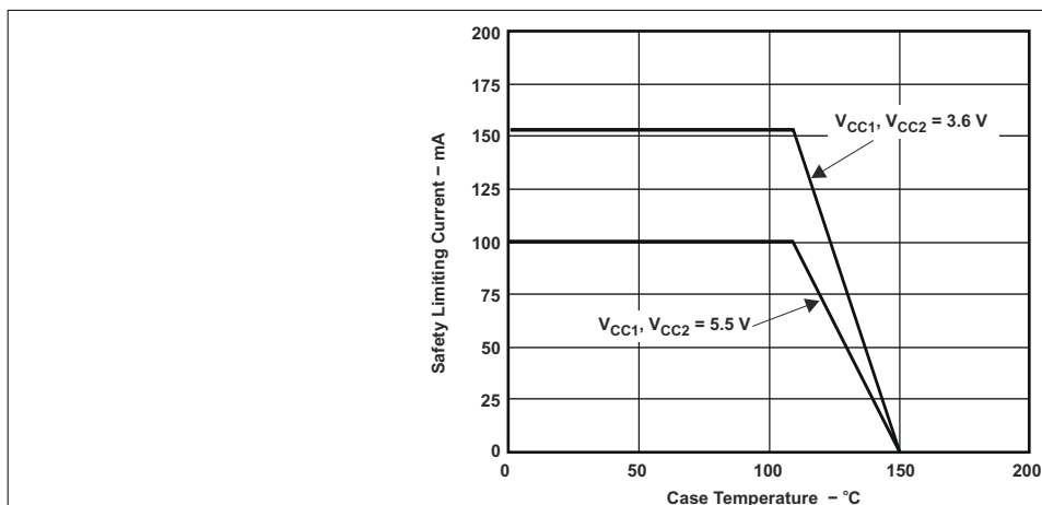
Figure 9-6. Thermal Derating Curve for Limiting Current per VDE
