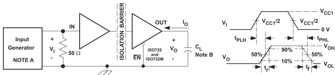
Figure 7-1. Switching Characteristic Test Circuit and Voltage Waveforms
