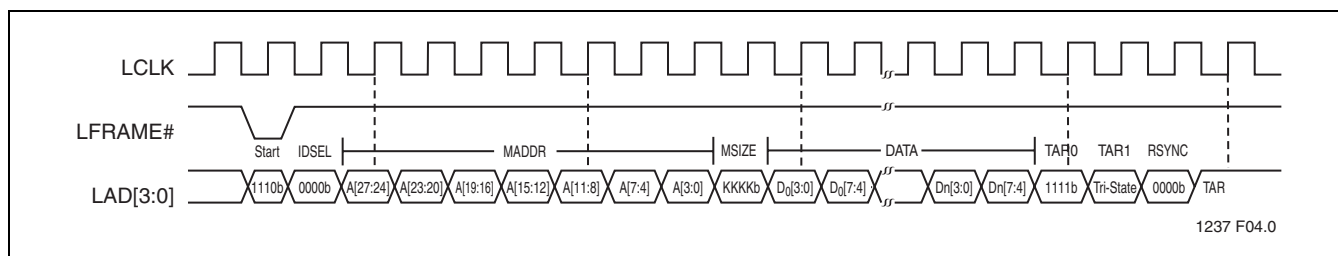
FIGURE 5: FIRMWARE MEMORY WRITE CYCLE WAVEFORM
