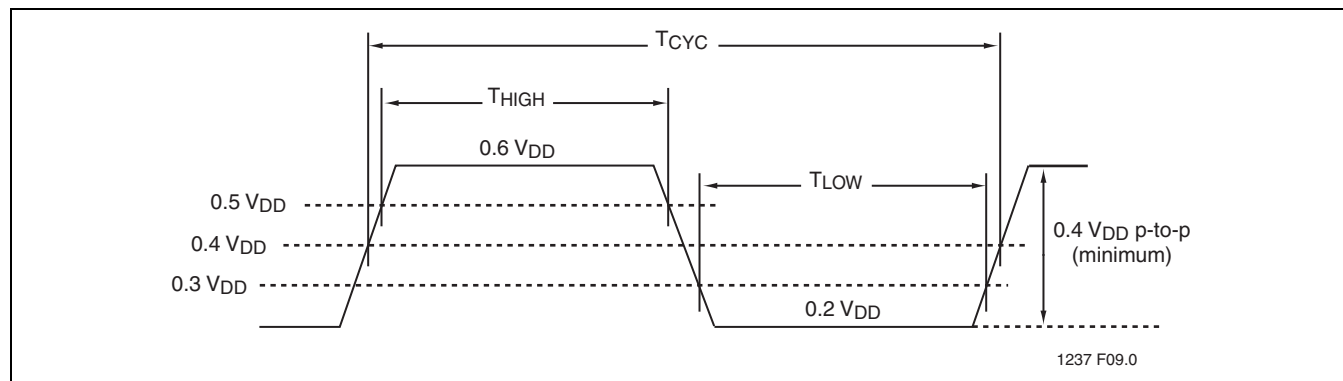
FIGURE 8: LCLK WAVEFORM (LPC MODE)
