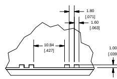
DETAIL B SCALE 1.50 : 1
