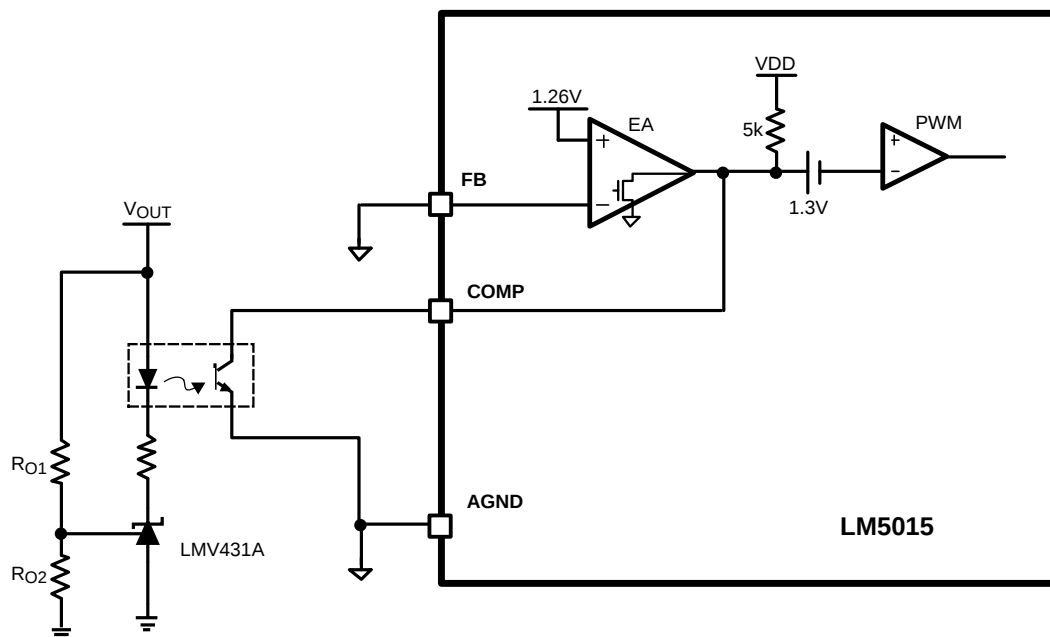
Figure 21. Conventional Isolated Feedback
