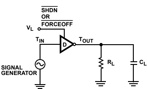
FIGURE 1A. TEST CIRCUIT
