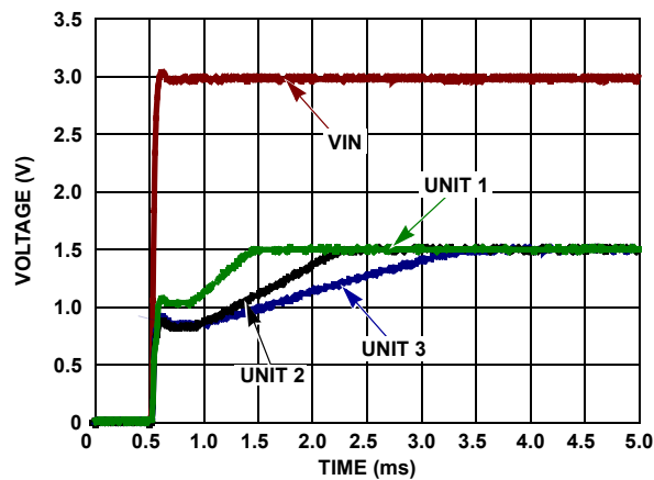
FIGURE 25. TURN-ON TIME
