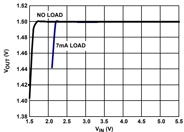
FIGURE 24. DROPOUT
