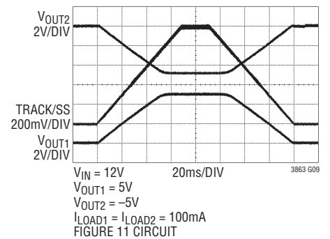
Output Tracking
