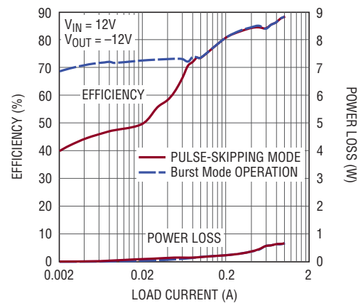
-12V Efficiency
