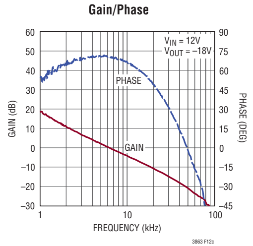
Figure 12. 5V to 23V Input, -18V/700mA Output, 750kHz Inverting Converter
