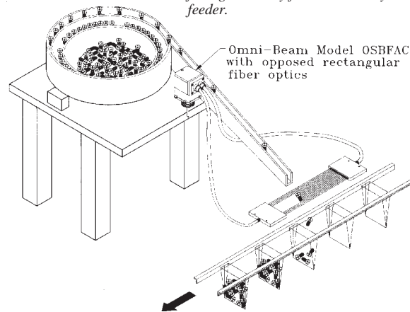
The OSBFAC detects small parts falling randomly from a vibratory feeder.
