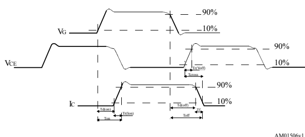
Figure 18. Switching waveform
