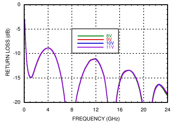
Input Return Loss vs. Vdd
