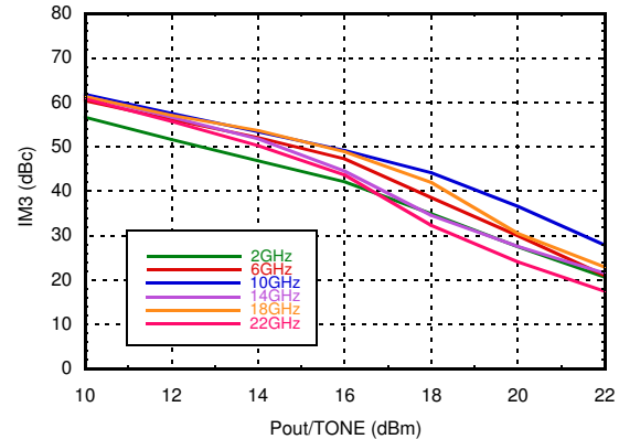
Output IM3 @ Vdd = +8 V
