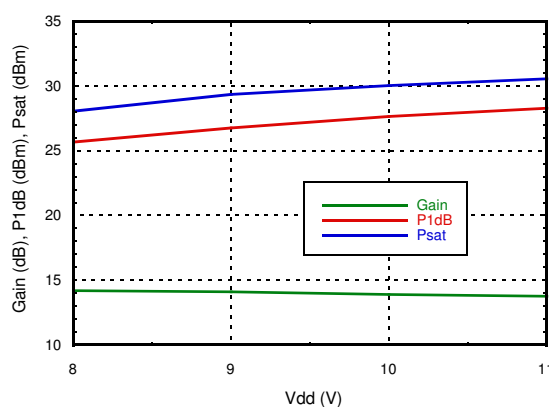
Gain & Power vs. Vdd @ 22 GHz
