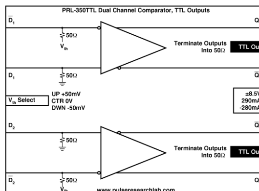
Fig. 1B PRL-350TTL Block Diagram
