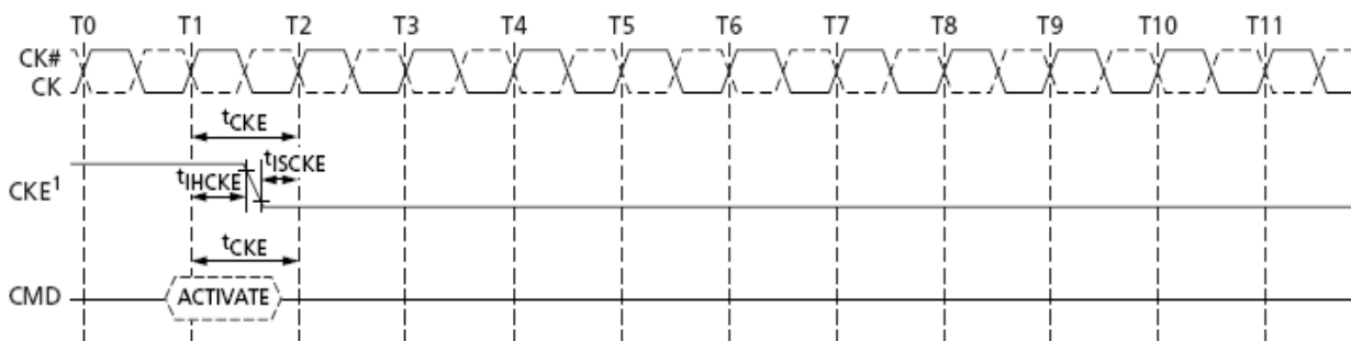
Activate command to Power-Down entry
