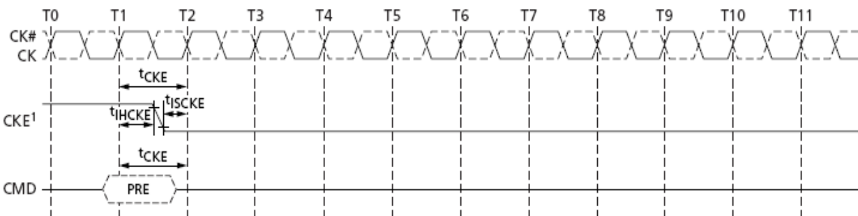
Precharge command to Power-Down entry
