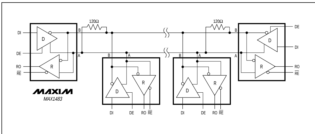
Figure 14. MAX1483 Typical Half-Duplex RS-485 Network
