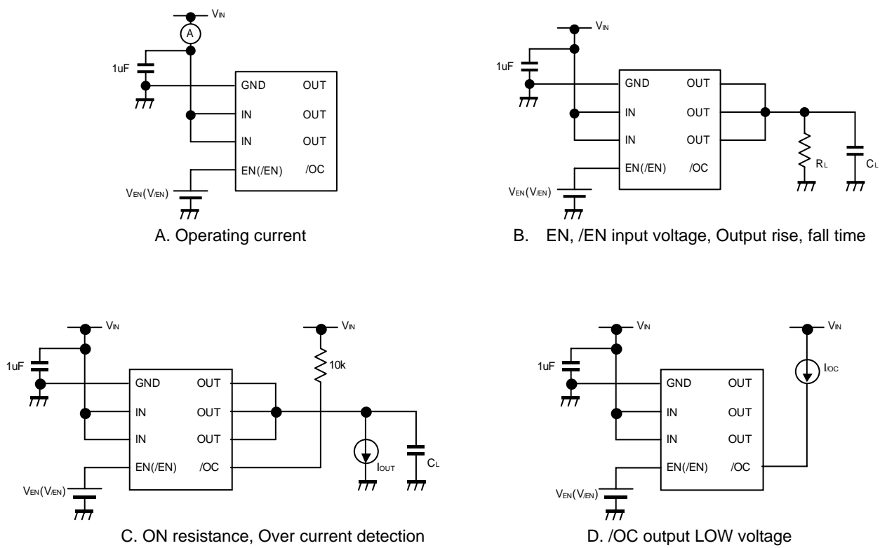
Figure 1. Measurement circuit
