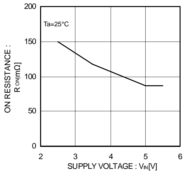
Figure 12. ON resistance
