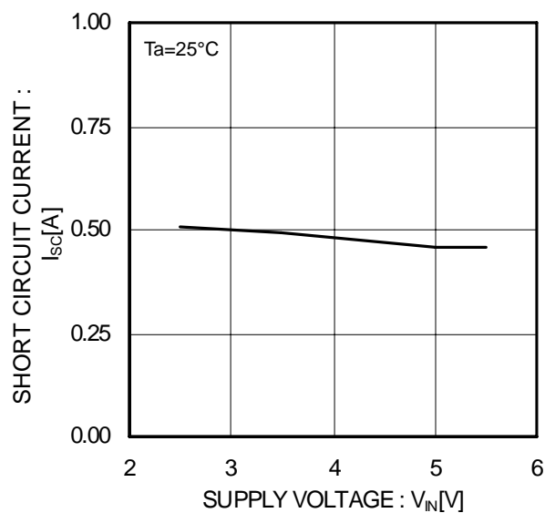
Figure 14. Output current at shortcircuit
