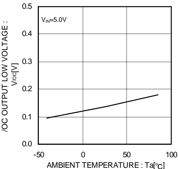
Figure 11. /OC output LOW voltage
