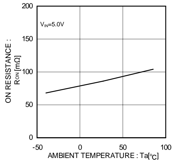
Figure 13. ON resistance
